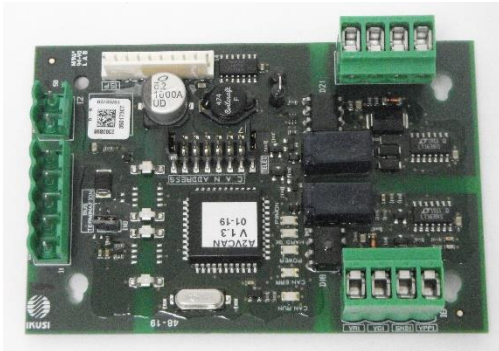
A2VCAN Analog Output Board
